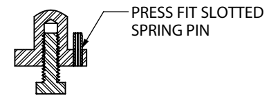
SECTION H-H
