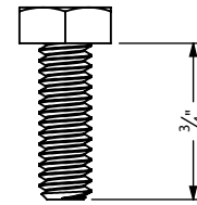
1/4-20 STEEL HEX HEAD MACHINE SCREW SCALE 1:1
