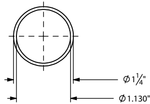
STEEL ANTENNA TUBE SCALE 1:2
